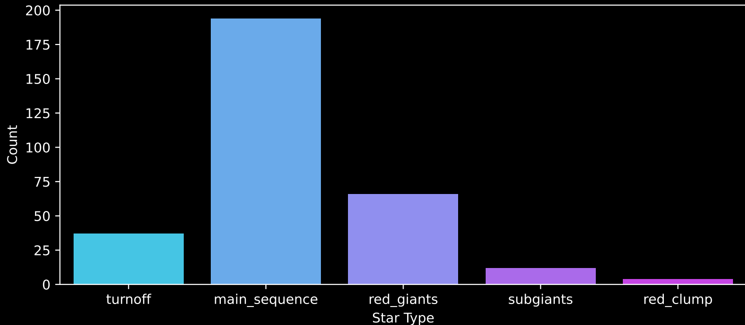
APOGEE DR17 Field: [293+62_btx] Count plot of Star Type
