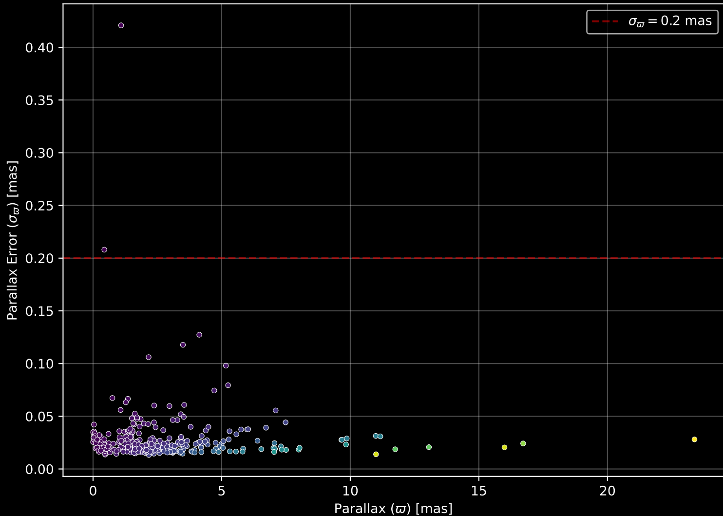
APOGEE DR17 Field: [293+62_btx] Parallax Quality (n= 313)
