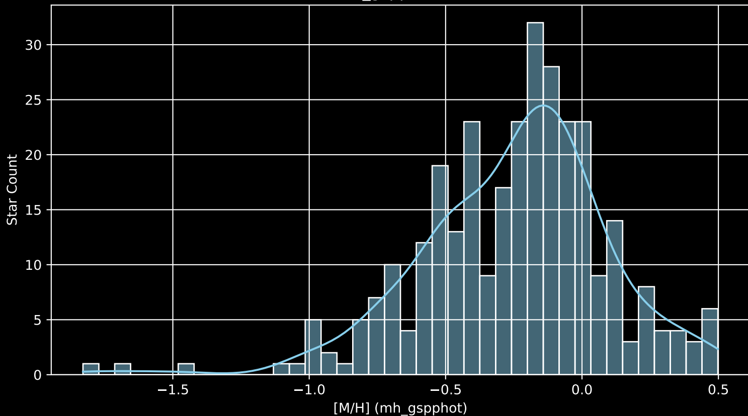
APOGEE DR17 Field: [293+62_btx [M/H] (mh_gspphot) (n= 312)
