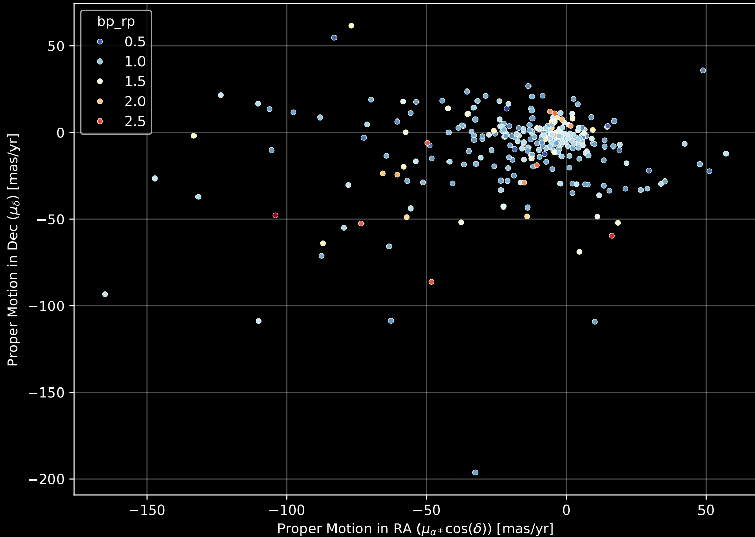
APOGEE DR17 Field: [293+62_btx] Proper Motion Diagram (n= 313)
