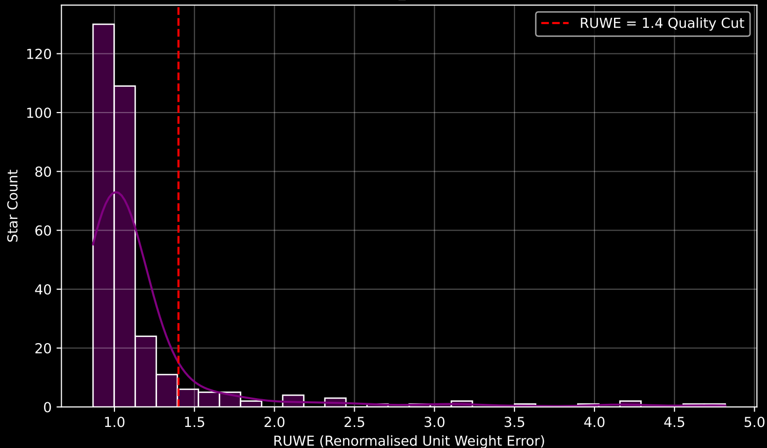
GAPOGEE DR17 Field [293+62_btx] RUWE Distribution (n= 310)
